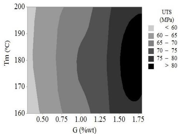
Fig. 6 2D interaction contour plots of graphene content (wt %) and temperature for ultimate tensile strength
