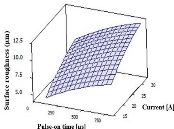
Fig. 6 Response surface of surface roughness in terms of current and pulse-on time
