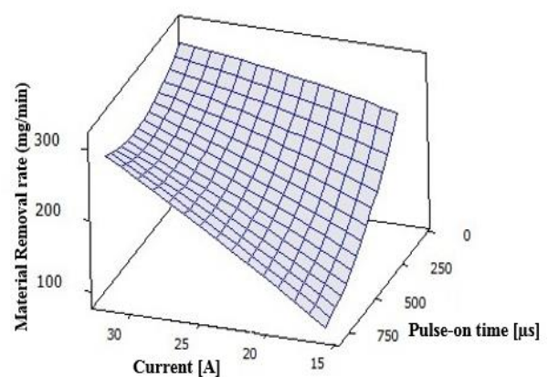
Fig. 5 Response surface of MRR in terms of current and pulse-on time
