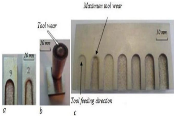
Fig. 8 a) tool wear effect on samples 2 and 9 b) tool wear effect on the electrode c) Tool wear comparison between samples
