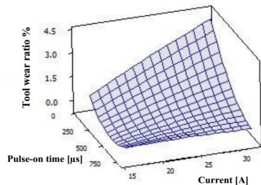
Fig. 7 Response surface of tool wear ratio in terms of current and pulse-on time
